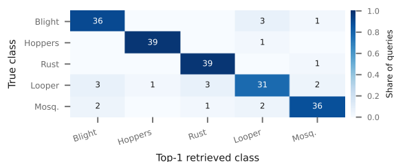
Fig. 8: Advisory retrieval confusion: true class against top-1 retrieved class, row-normalized so the diagonal is per-class precision@1; cells are query counts. Looper caterpillars is the weak row (31/40); hoppers and rust retrieve almost perfectly.
