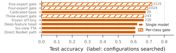
Fig. 5: The image-only ladder. Rungs are alternative methods rather than stages of one progression, so they are compared as bars rather than joined by a line; the search size each rung fitted is annotated. Accuracy rises 0.613 to 0.720 across three decades of search. The ladder carries no note axis because the image branch does not move when notes are deleted. Hatched bars are per-class gates, which are diagnostics rather than deployable models.
