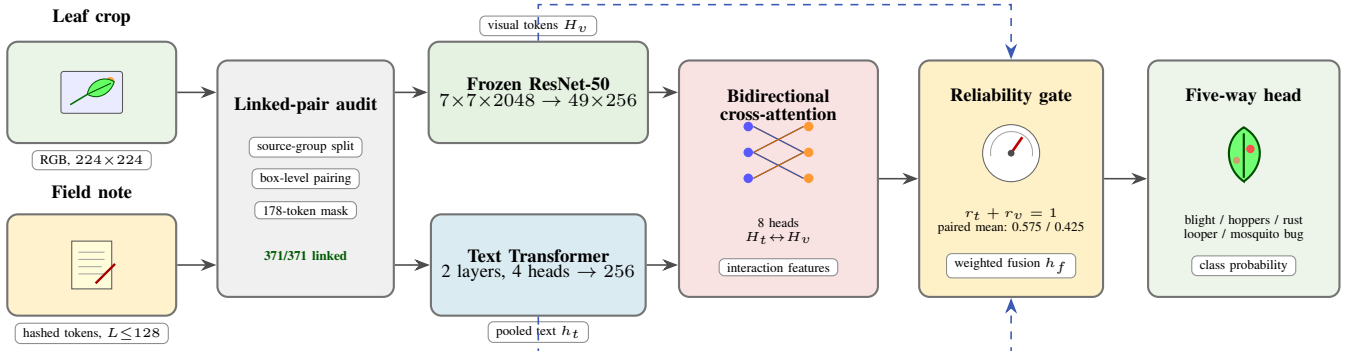
Fig. 2: Clip-art view of the active inference architecture. Exact box-level linkage and the training-fitted target-token mask precede the two encoders. Visual and textual tokens interact through bidirectional cross-attention; a learned reliability gate then weights the two parents before five-way classification. Dashed paths are the two unimodal expert heads, which re-enter the prediction at inference as a reliability-weighted residual and also carry auxiliary training losses.
