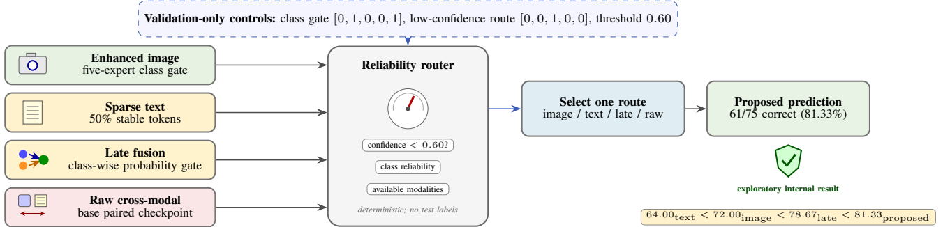
Fig. 3: Clip-art view of reliability-aware sparse-note inference. Four available prediction routes feed a deterministic router whose class gate, confidence threshold, and low-confidence action are selected on validation. The accuracy ladder is an exploratory internal observation; the router does not read test labels and the result is not pristine external evidence.
