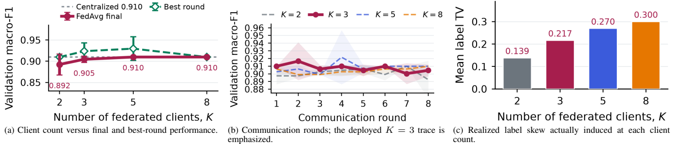
Fig. 4: Measured multimodal FedAvg adaptation on the source-disjoint tea validation split. Points are macro F1 mean \pm standard deviation over three client-partition seeds; 222 training crops, 74 validation crops, \alpha = 1 , one local epoch, full participation, and a frozen ResNet-50 are fixed. The dotted line in (a) is the 0.9099 initialization, and (c) is the realized label total variation, so (a) is read against measured rather than assumed skew. The 75-crop test is not used, and client ownership is simulated rather than estate-derived.
