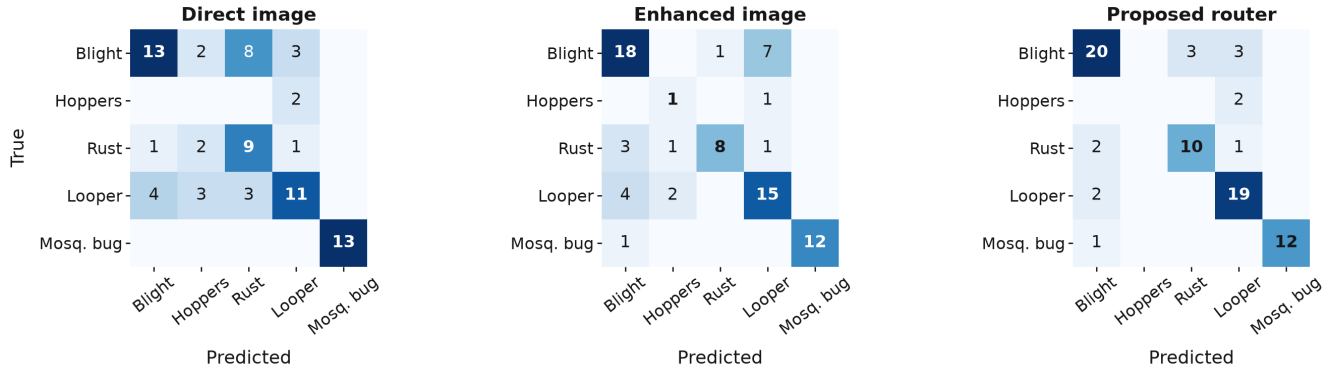
Fig. 7: Where the errors land on the fixed 75-crop test. Each matrix sums to 75; diagonals give the 46, 54, and 61 correct crops of the direct image path, the five-expert enhanced gate, and the exploratory router. The off-diagonal cells are the part no count table records: leaf blight is confused with rust and looper rather than scattered, looper recovers most under the router, and the two leaf-hopper crops fall into looper except for one the enhanced gate recovers.
