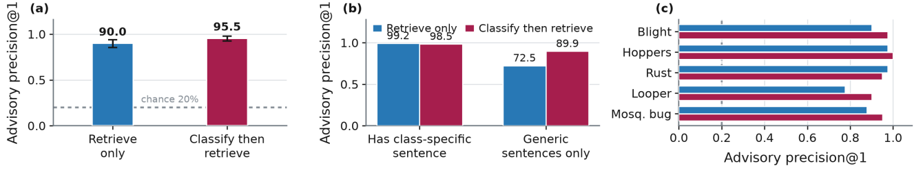
Fig. 6: Measured Classify–Retrieve–Advise quality on the templated symptom corpus: 472 passages, 201 queries, exact inner-product search. (a) Precision@1 with bootstrap intervals against chance; (b) split by whether the query holds a class-unique sentence; (c) per class. Same five classes as the diagnostic experiments, but a different corpus and support, never pooled with them.
