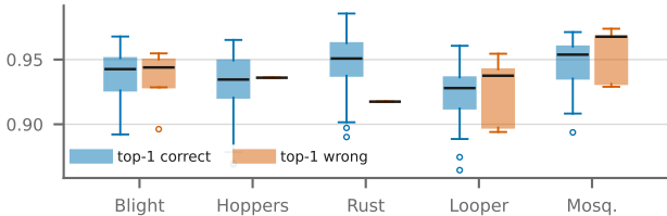
Top-1 similarity
