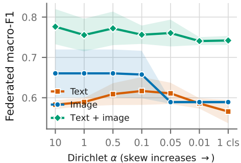
(a) Severe label skew
