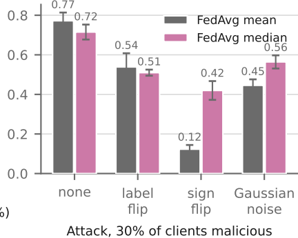
(c) Poisoned updates (fusion)
