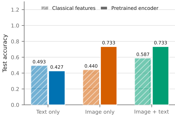
(a) Classical vs. pretrained, 50% of notes deleted
