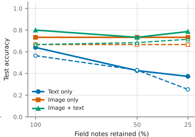
(b) Centralized (solid) vs. federated (dashed)
