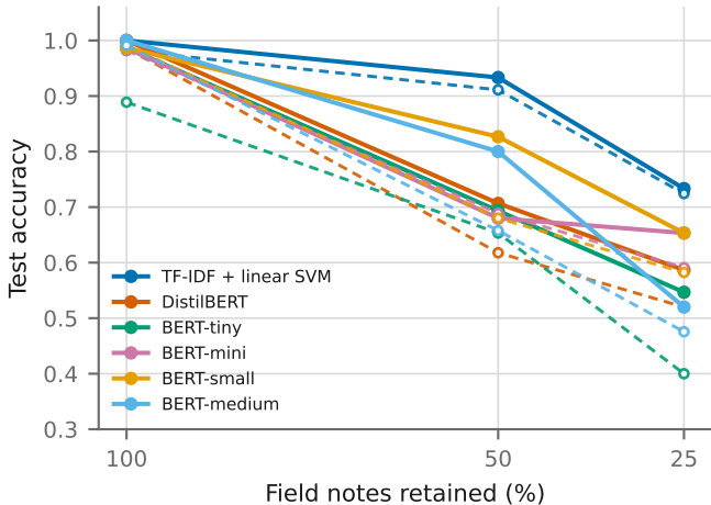
Text encoders as notes are deleted
