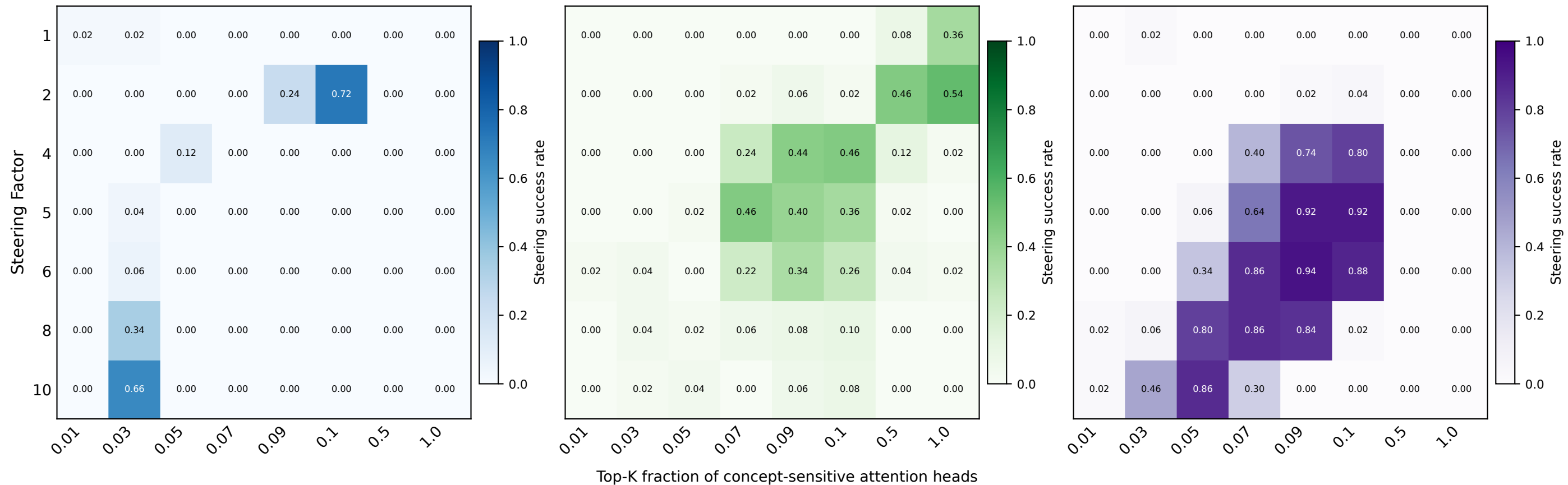
Localization: Verse (Long) · Long-Form Eval, Long-Form Steer · w/ R+F Filter Qwen 1.5-14B OLMo 2-13B Qwen 1.5-32B
