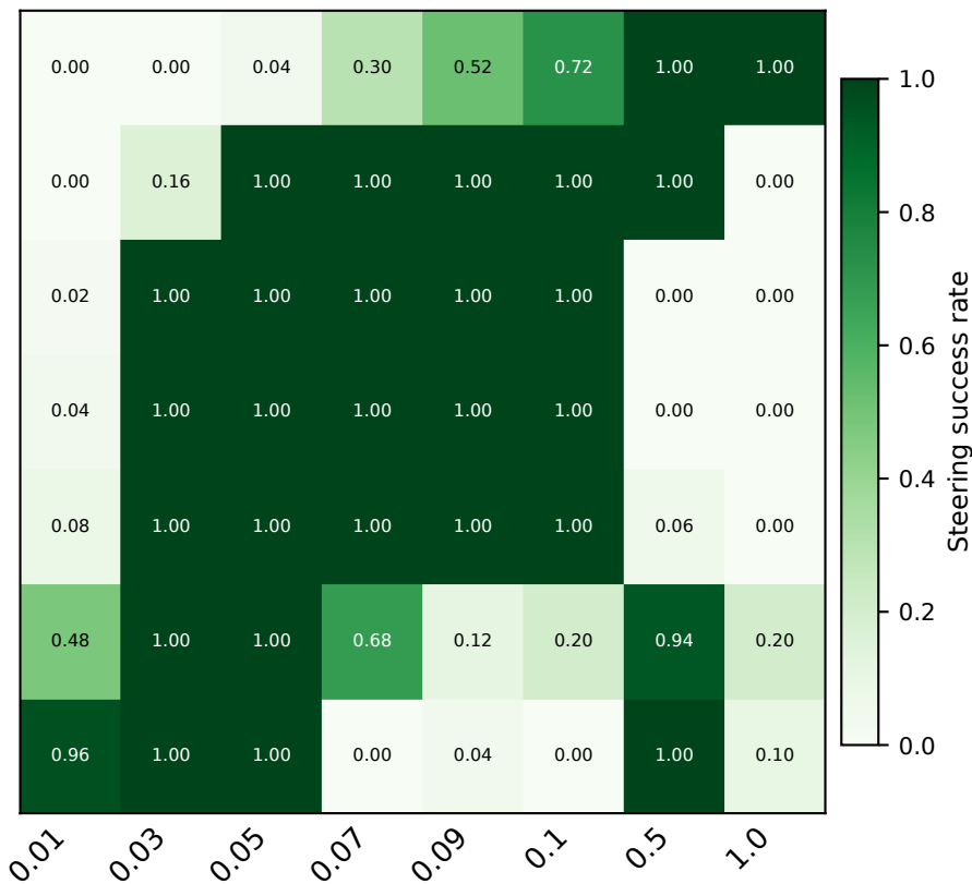
Sycophancy (Single) · Single-Token Eval, Single-Token Steer · Token Matching
