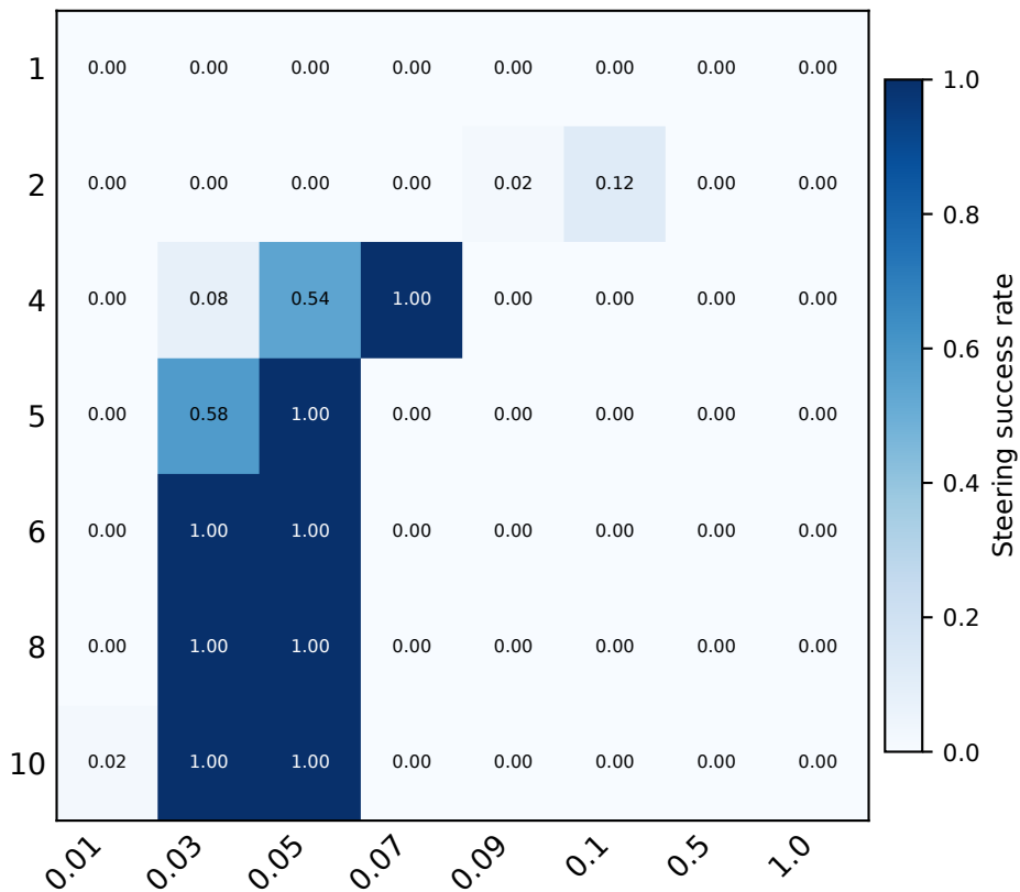
Sycophancy (Single) · Single-Token Eval, Single-Token Steer · Token Matching
