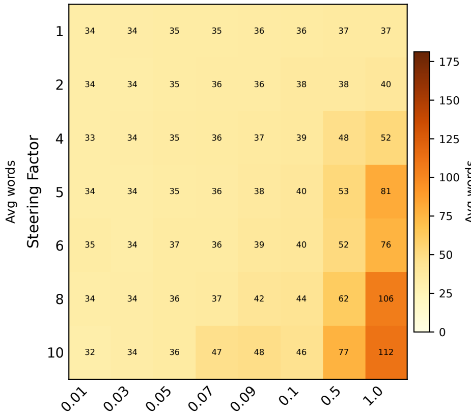
Summarization (Long Loc) · Long-Form Eval, Single-Token Steer · Avg Word Count OLMo 2-13B Qwen 1.5-32B Gemma 3-12B
