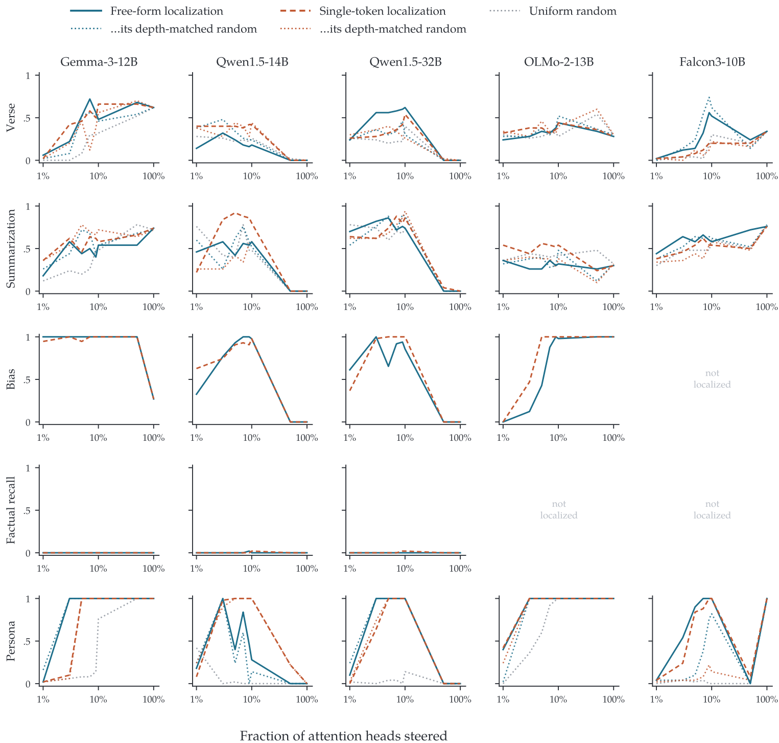
Localization on single-token evaluation, per task and model
