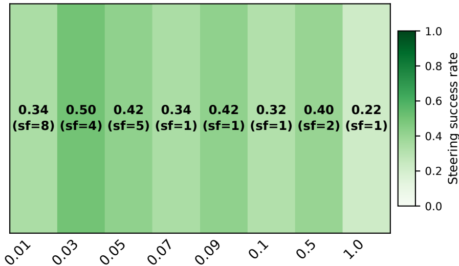
Summarization (Long) · Single-Token Eval, Single-Token Steer · Token Matching Qwen 1.5-32B
