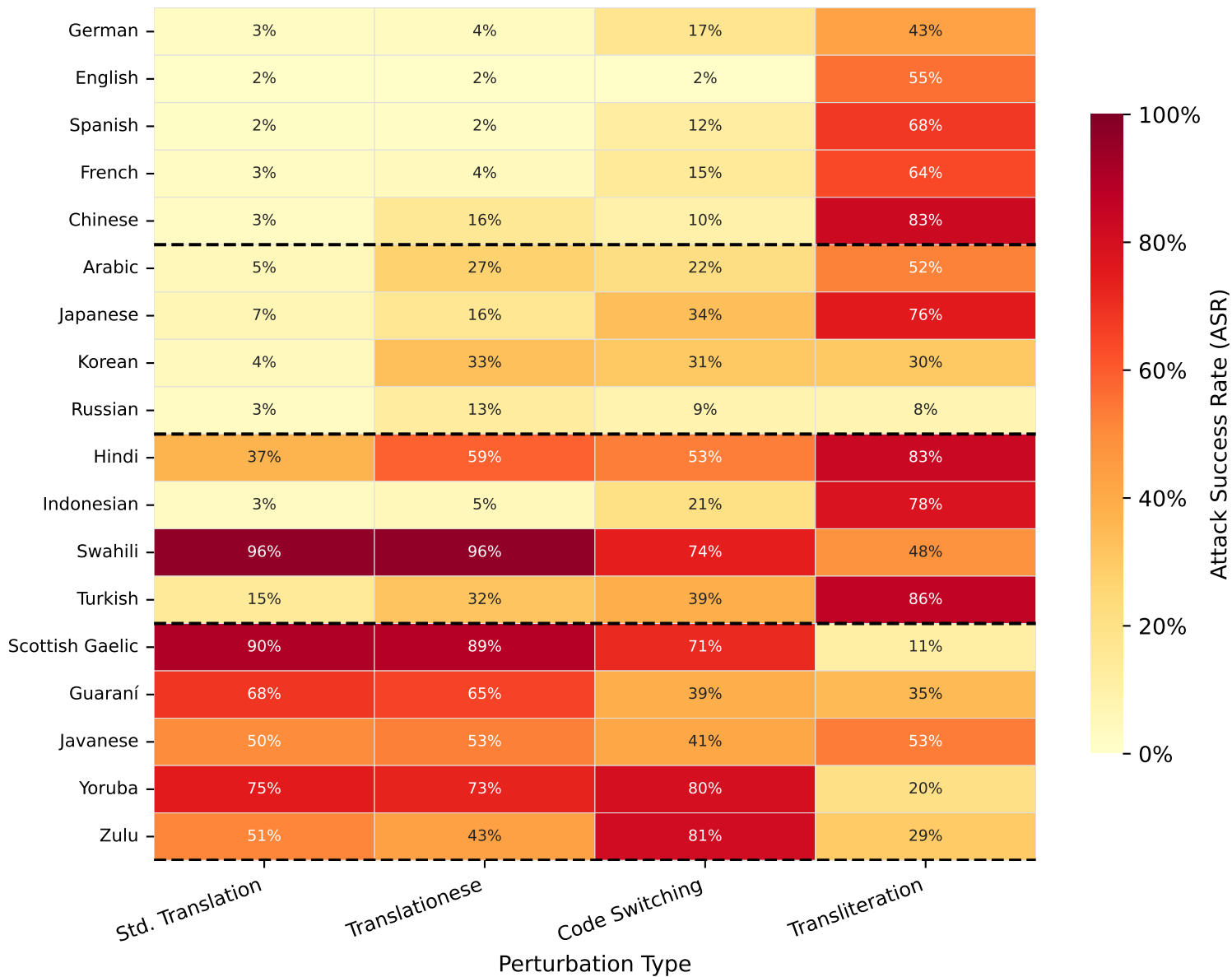
ASR Heatmap — Qwen2.5-7B-Instruct
