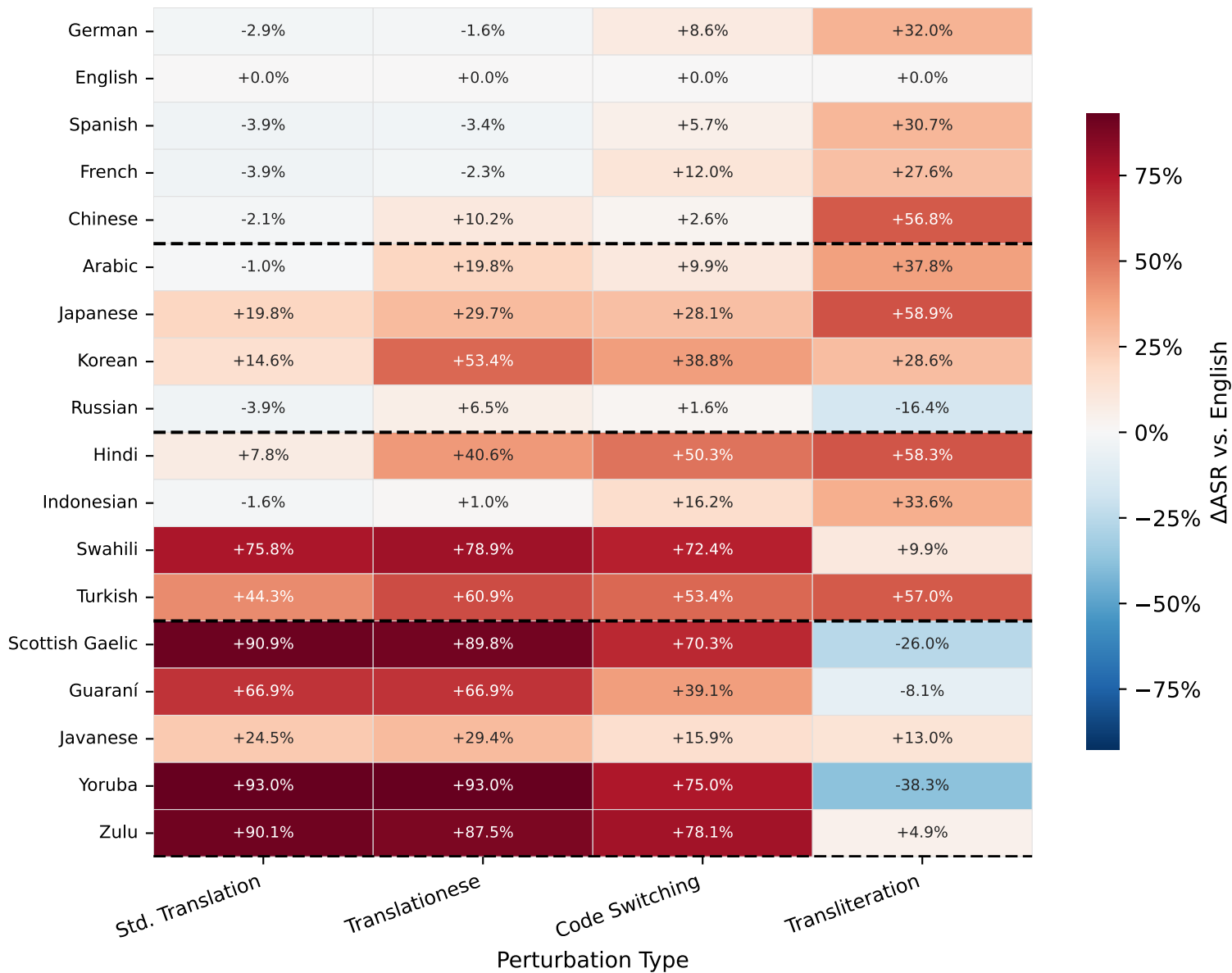
\Delta ASR from English Baseline — Llama-3.1-8B-Instruct
