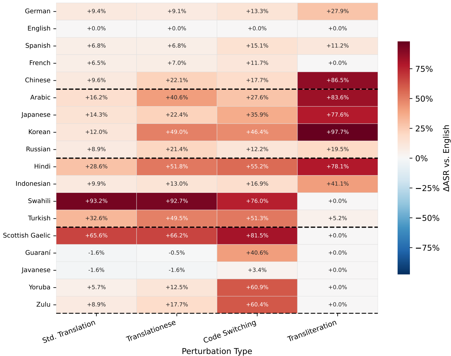
\Delta ASR from English Baseline — aya-expanses-8b
