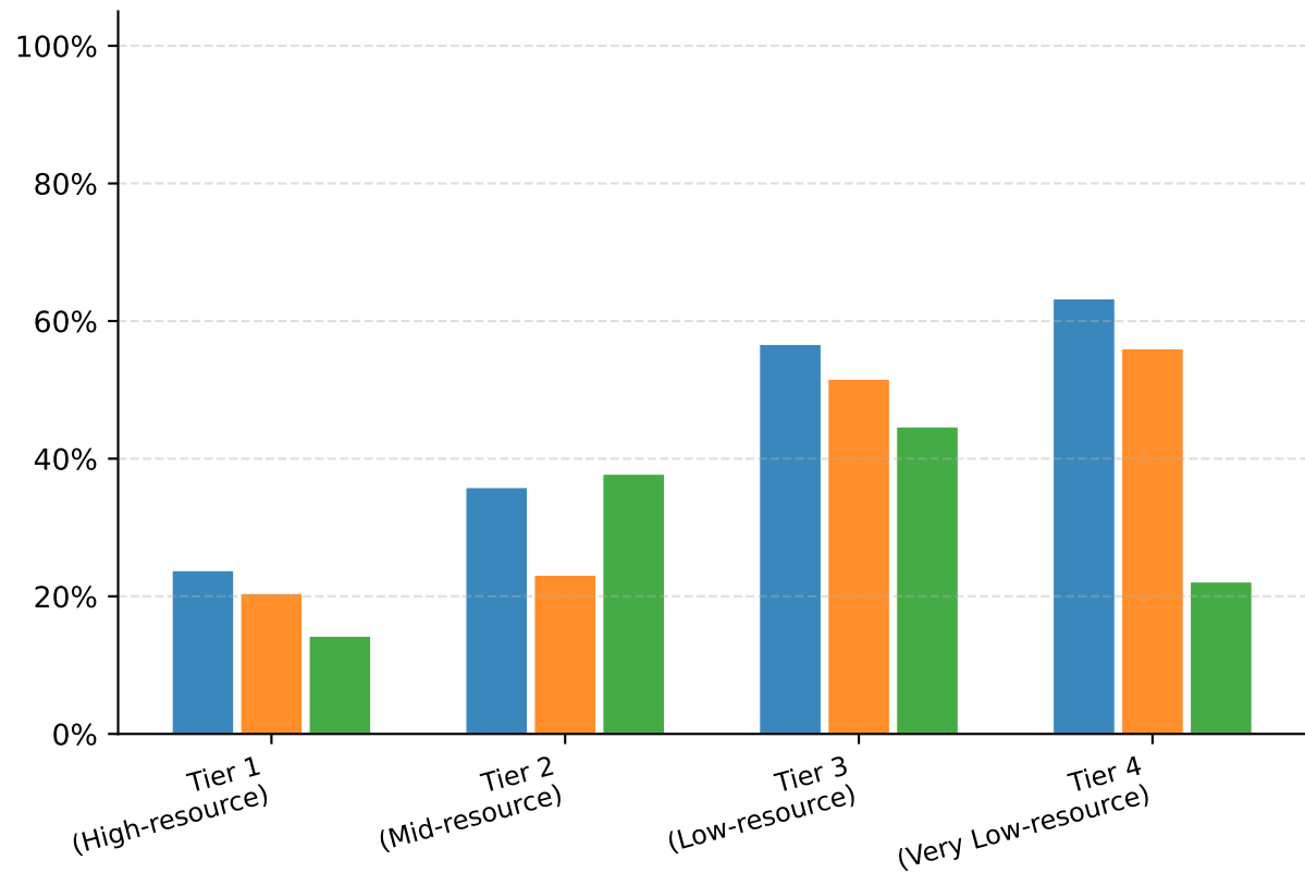
Mean ASR by Language Tier
