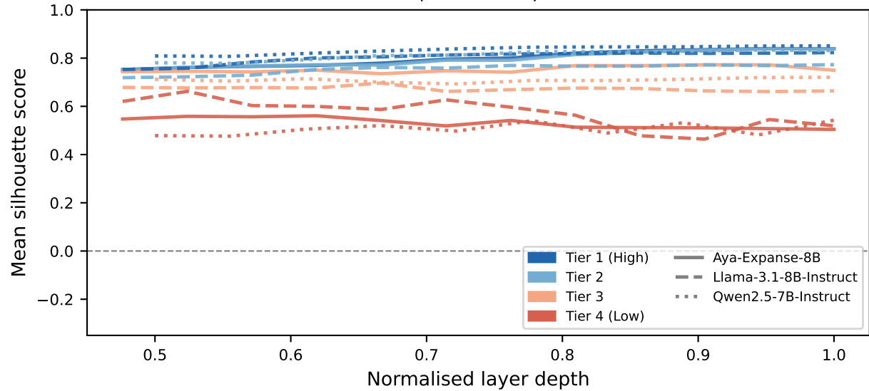
Tier-Averaged Separation Across Layers (all models)
