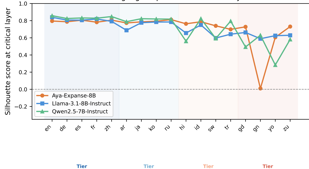
Per-Language Separation at Critical Layer
