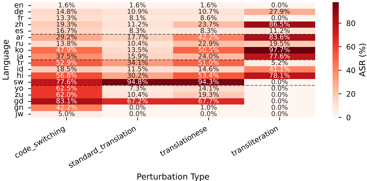
Attack Success Rate — aya-expanse-8b
