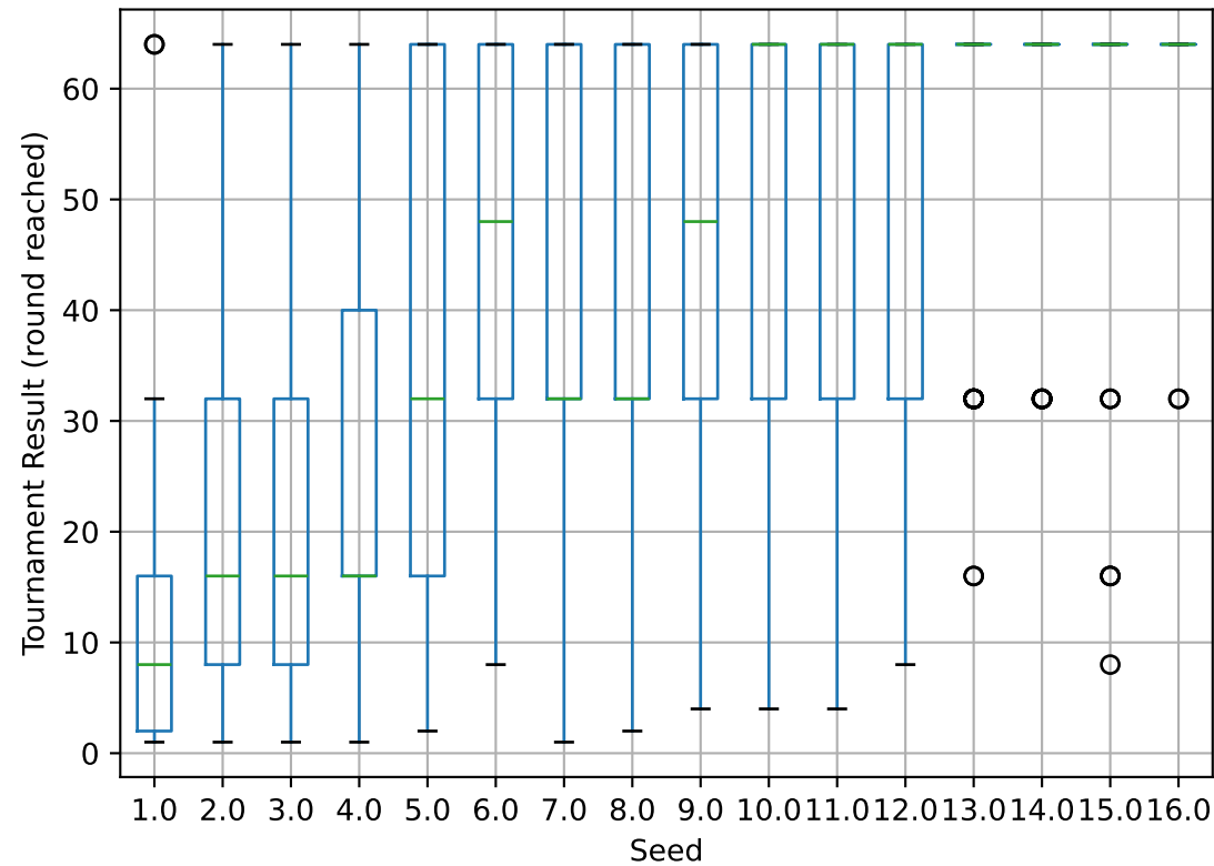
Distribution of Results by Seed
