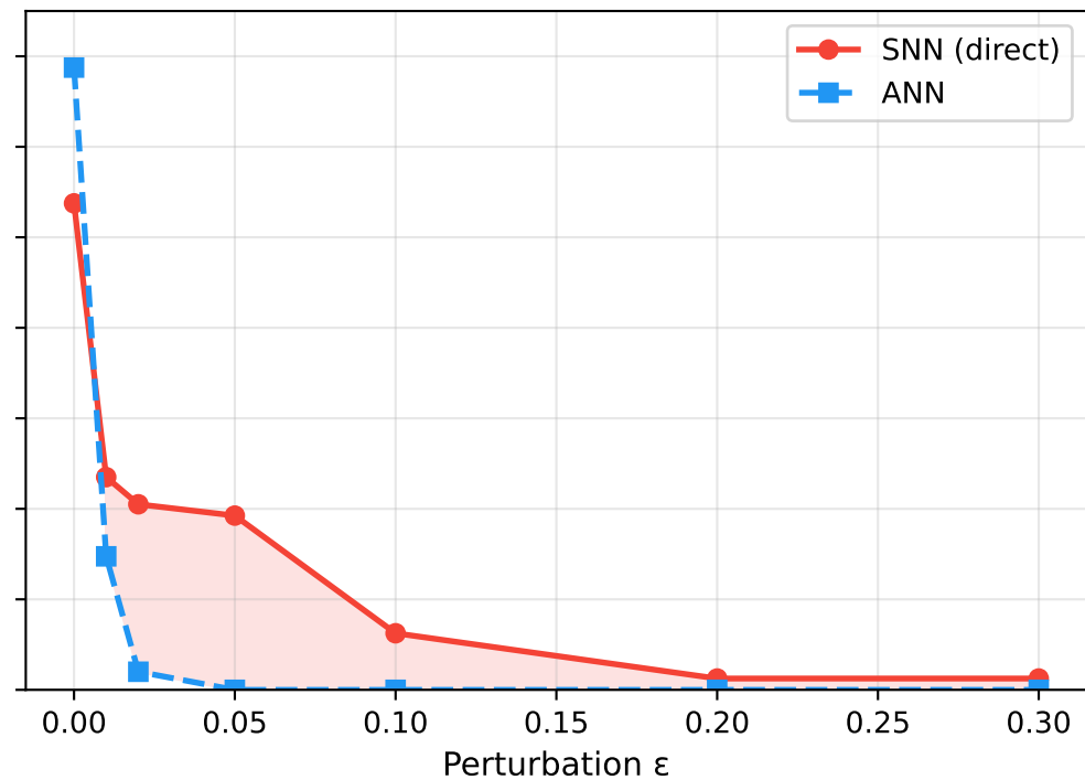
PGD Attack
