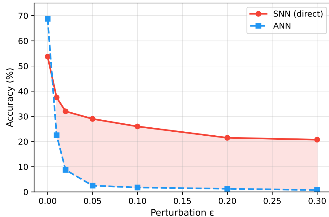
FGSM Attack
