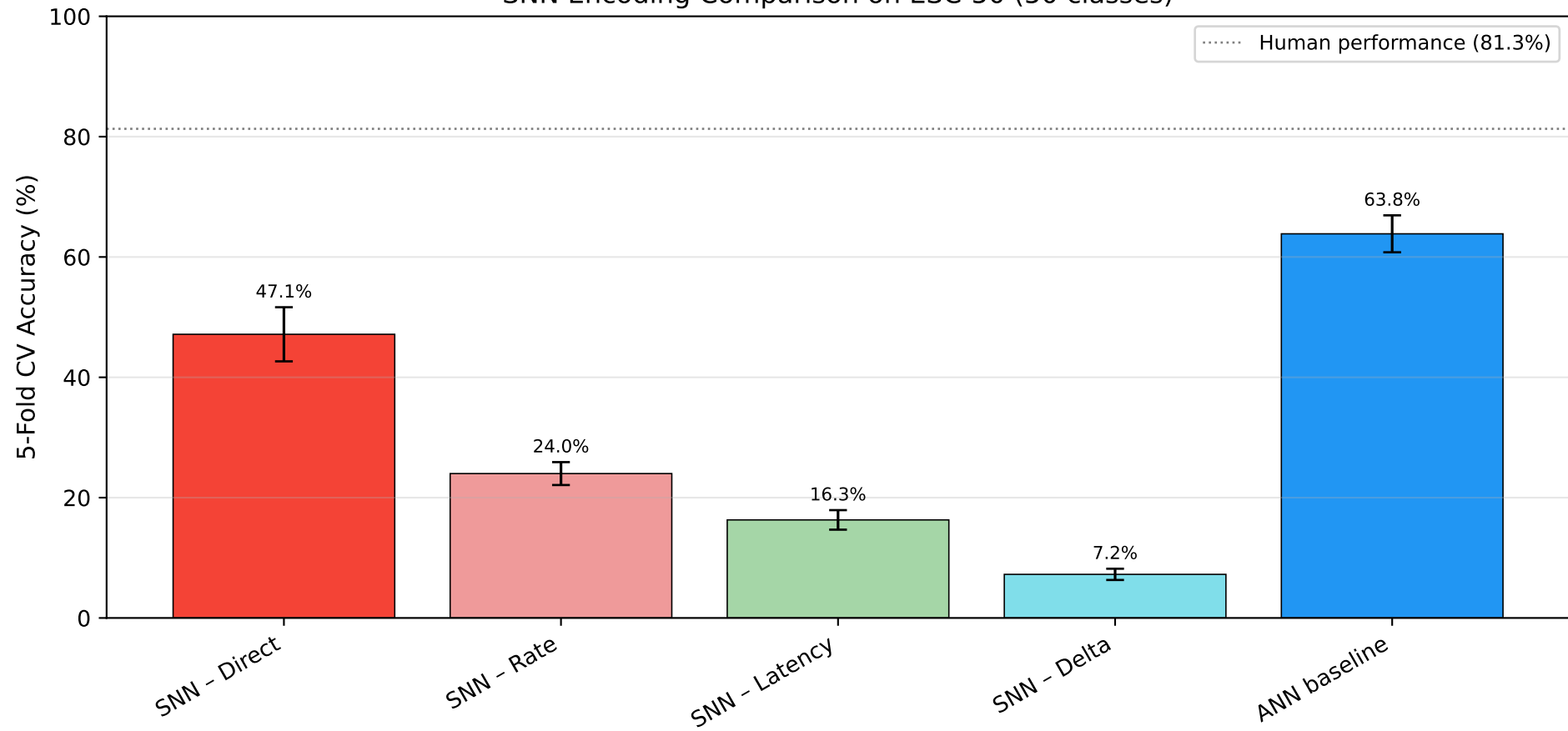
SNN Encoding Comparison on ESC-50 (50 classes)
