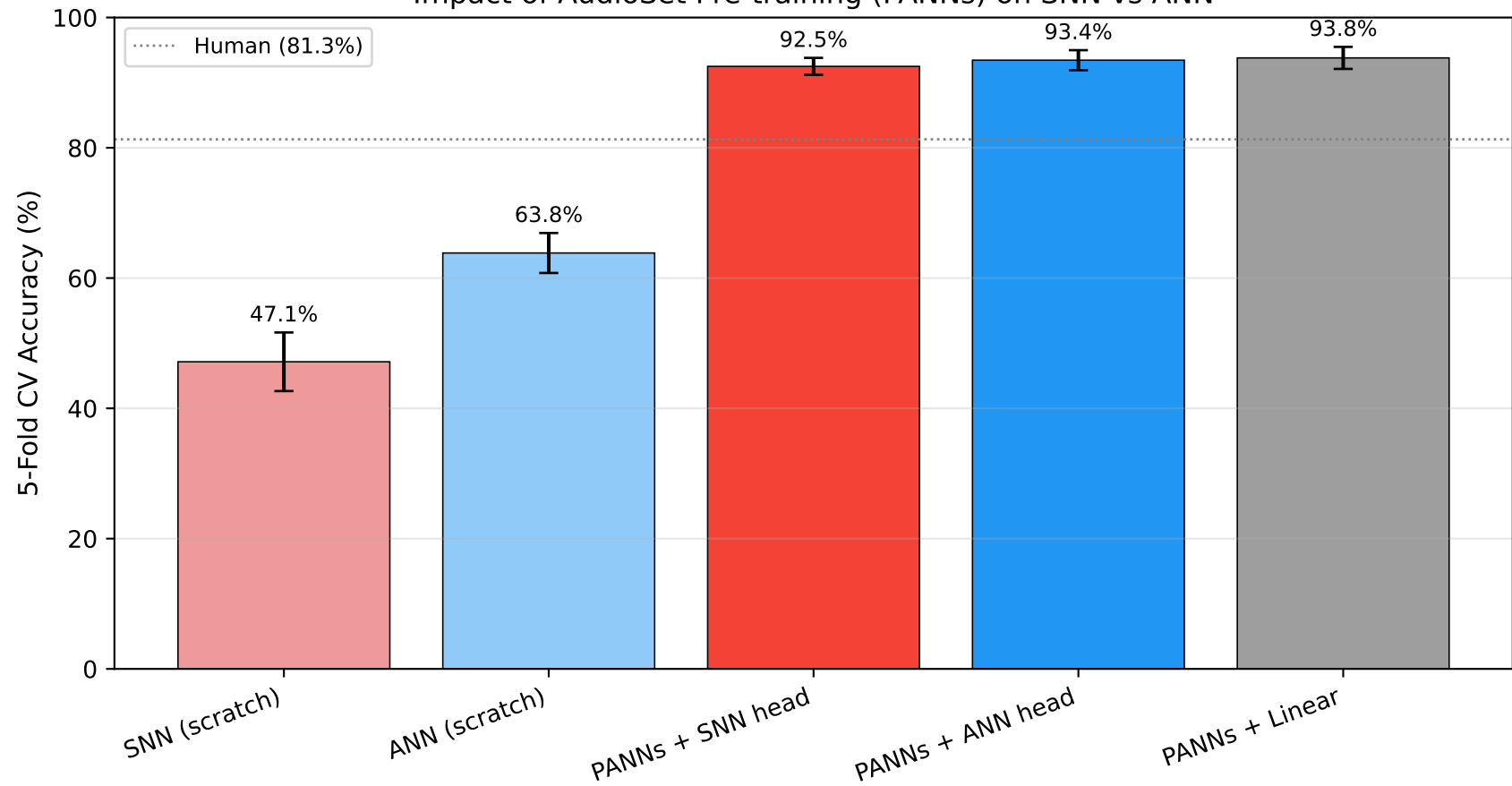
Impact of AudioSet Pre-training (PANNs) on SNN vs ANN
