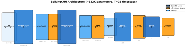
Figure 1: SpikingCNN architecture. The ANN baseline replaces each LIF with ReLU. Both have ~622K parameters.
