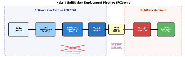
Figure 2: Hybrid SpiNNaker deployment pipeline. Full deployment failed because AvgPool outputs are fractional, causing excitatory-inhibitory cancellation in \text{FC}_1 (see Section 4.3).
