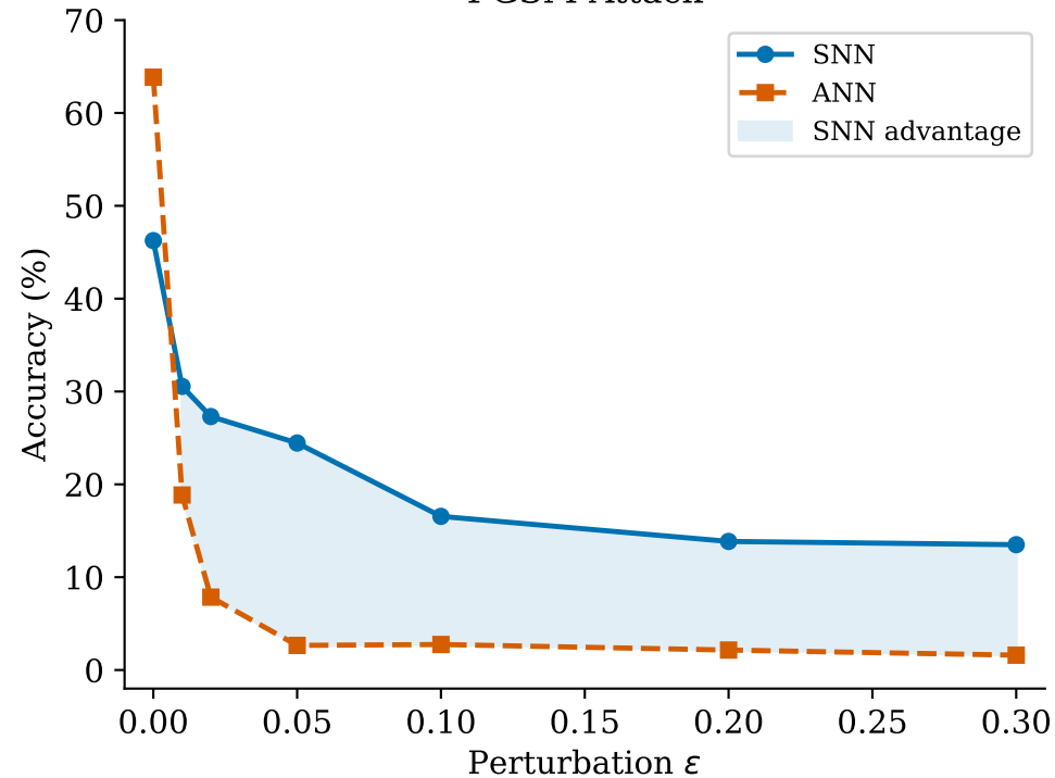
FGSM Attack
