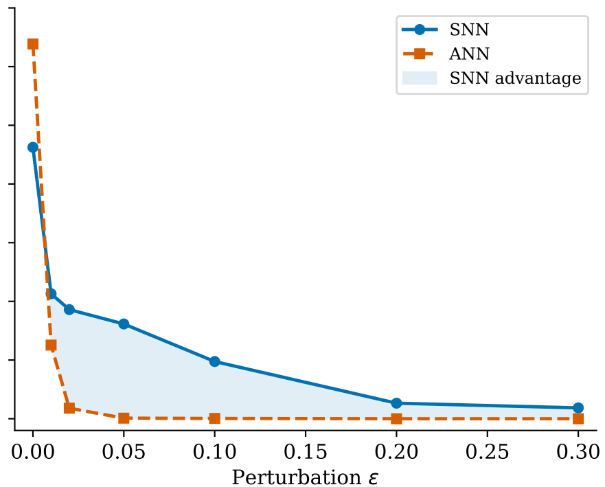
PGD Attack
