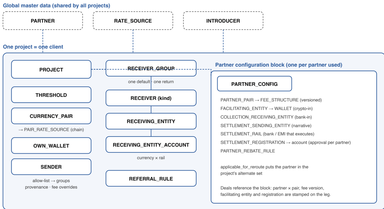
Figure 1 — The configuration model. Dashed boxes are global; everything inside the shaded area belongs to one project.
