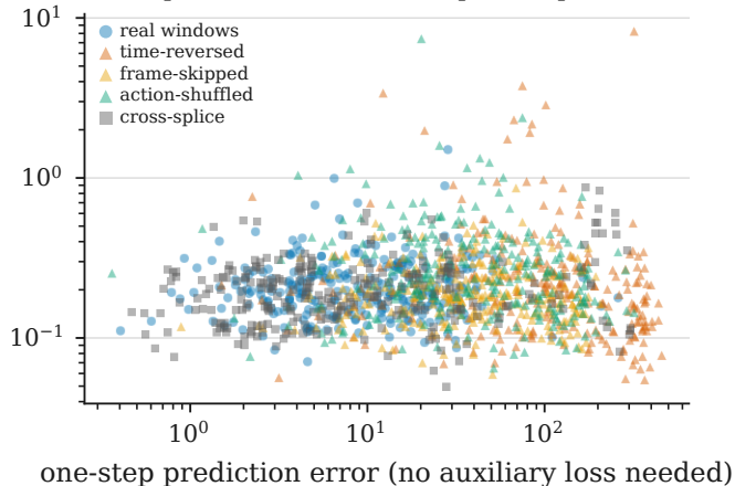
(b) sequences: \delta does NOT separate; prediction error does
