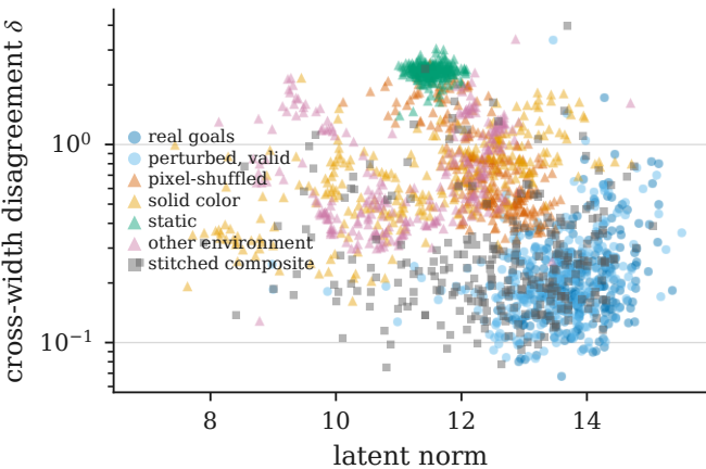
(a) goal images: not a diagonal (Spearman -0.55 )
