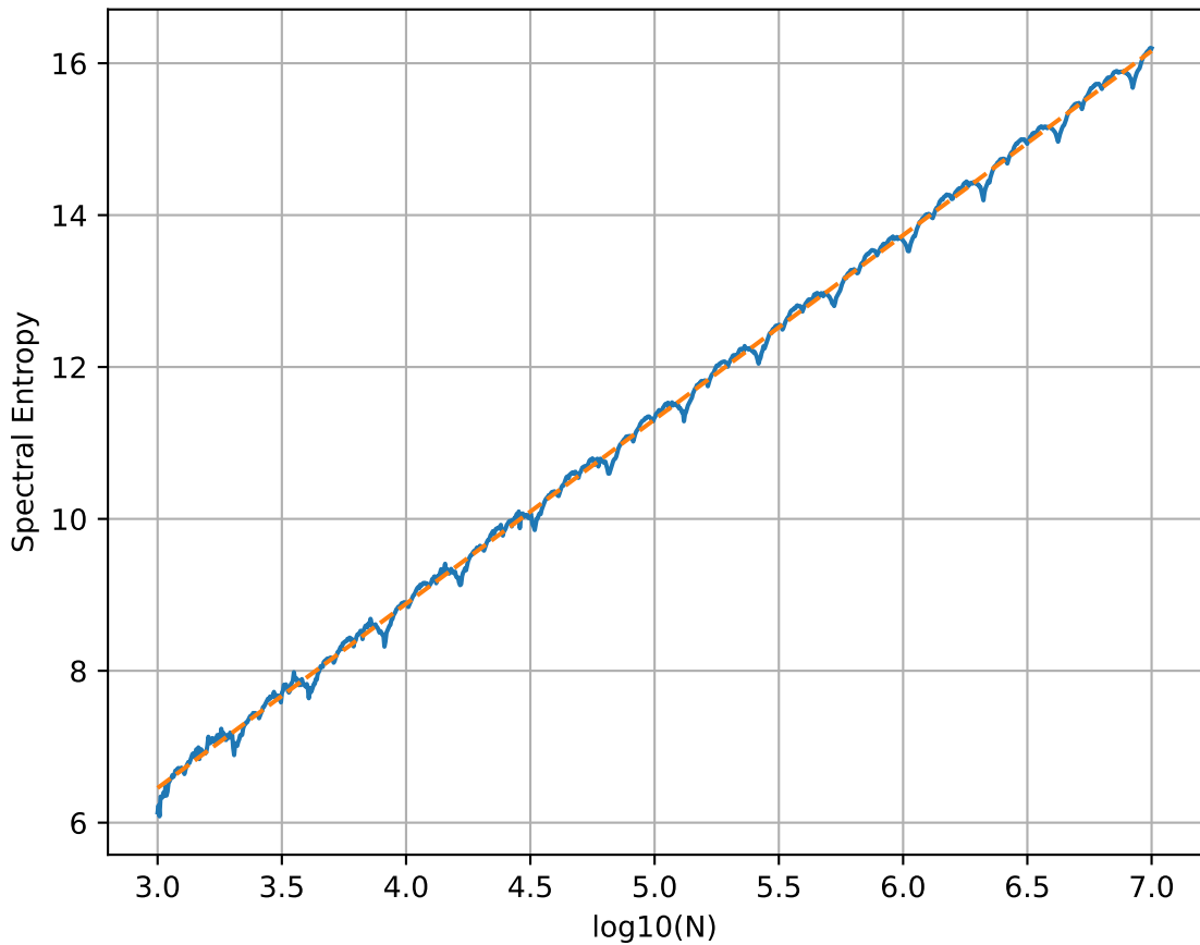
thue - Spectral ( \alpha=2.427 )
