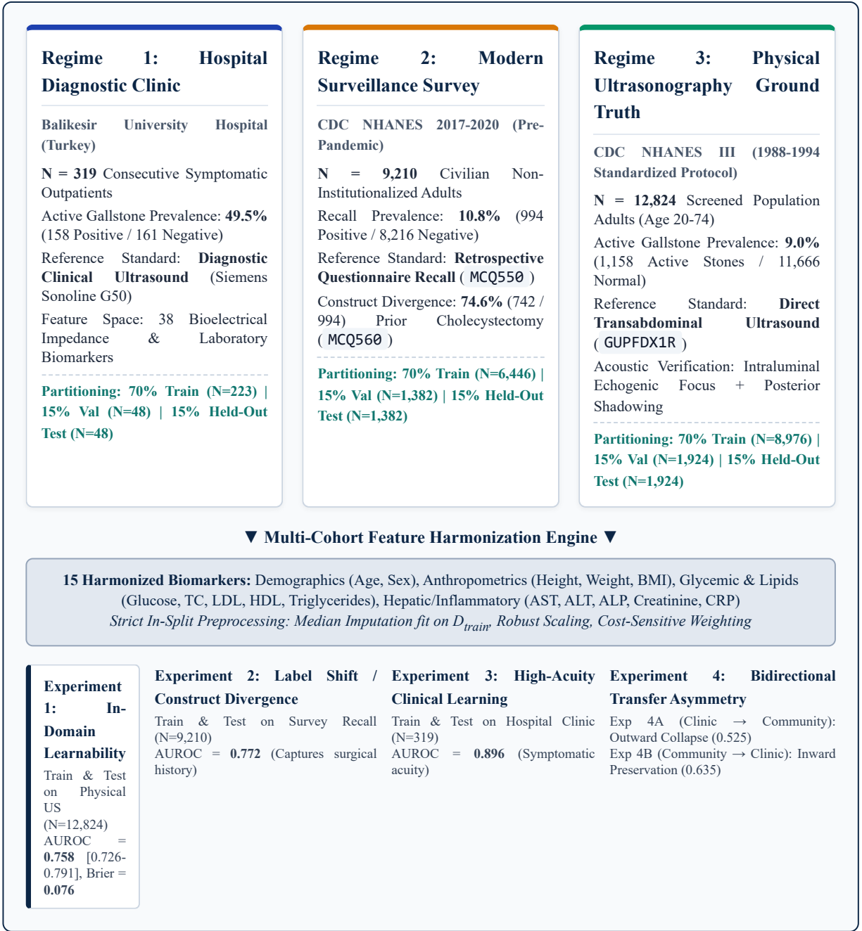
Figure 1: Multi-Cohort Conceptual Architecture, Epidemiological Regimes, and Patient Flow Diagram. Regime 1 (High-Acuity Diagnostic Clinic, N = 319 , active prevalence 49.5%), Regime 2 (Modern Civilian Surveillance Survey, N = 9,210 , recall prevalence 10.8%), and Regime 3 (Nationwide Standardized Physical Ultrasonography Ground Truth, N = 12,824 , active prevalence 9.0%), harmonized across 15 standardized clinical biomarkers.
