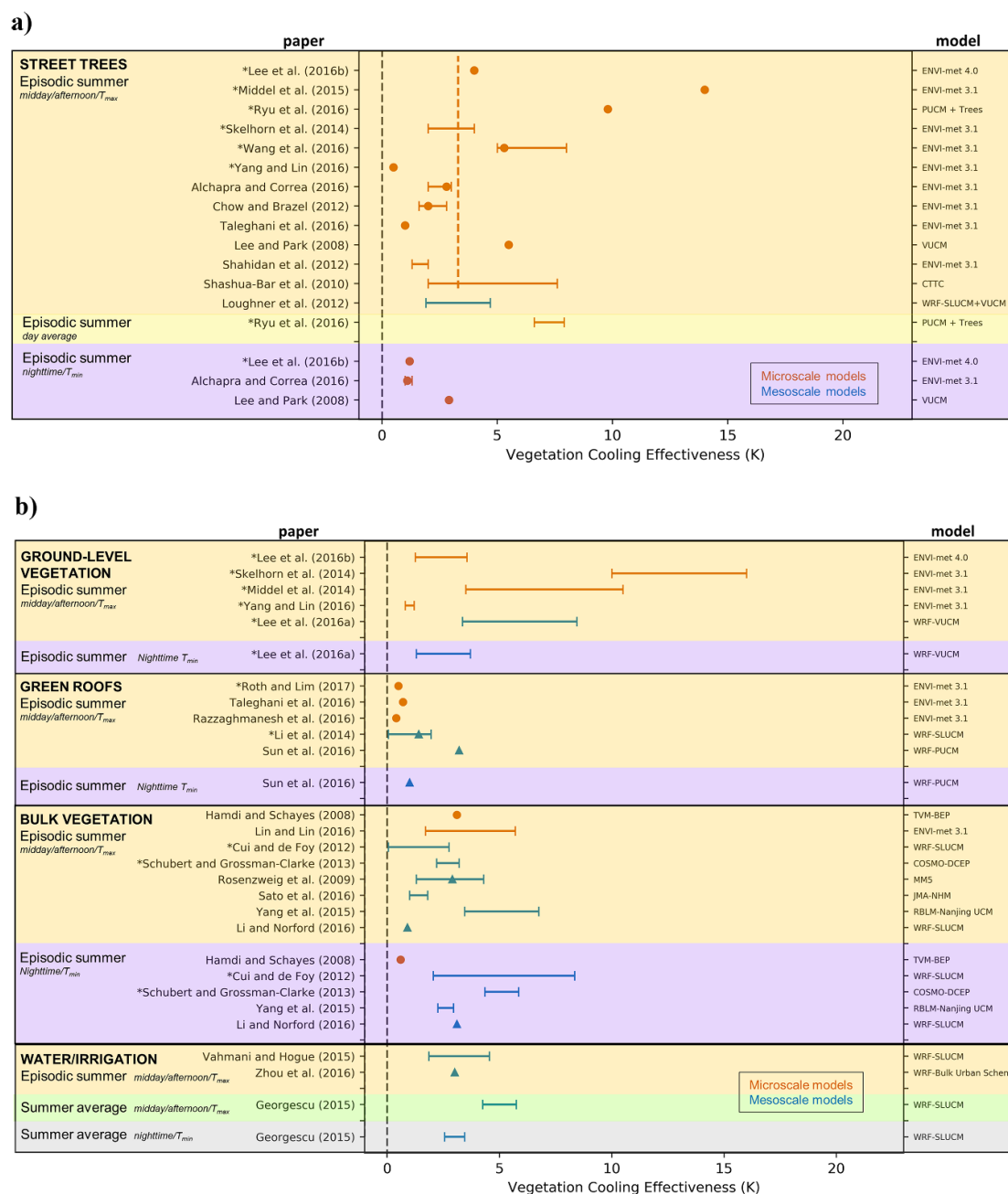
Figure 7. Vegetation cooling effectiveness (VCE) from street tree (a) and other (b) vegetation implementations for two model scales and across several seasons and approximate times of day. Symbols are as in figure 6. Vertical, orange dashed lines in (a) indicate median ACE for summer afternoon microscale study results.
