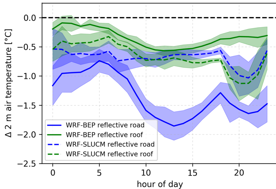
Figure 8. The importance of model physics representations of urban surface layer exchange on air temperature cooling from albedo enhancement. A diurnal composite of cooling during a 2006 heatwave in Phoenix studied by Broadbent et al (2020a) is plotted for two urban canopy models (UCMs) embedded in the WRF mesoscale model. For each UCM, the albedo of road and roof are increased in separate simulations to 0.88.
