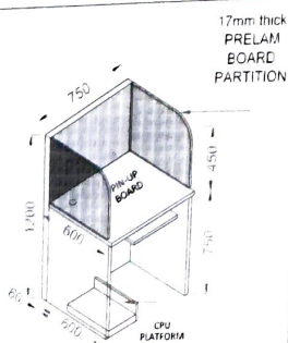
WALL SIDE MODULAR WORKSTATION
