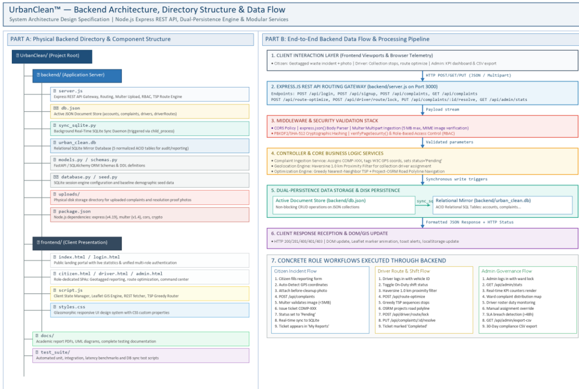
Figure 5.13: UrbanClean Backend Structure and Data Flow
