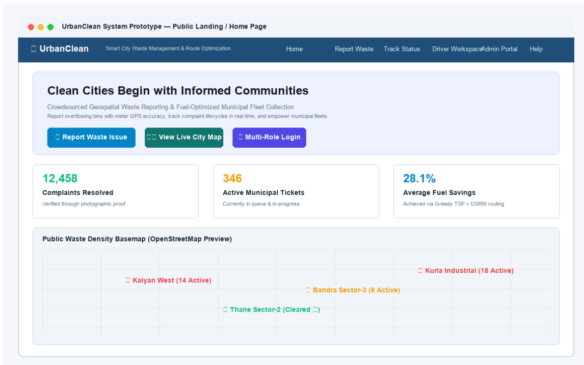
Figure 5.1: Prototype — Public Landing Page & Cleanliness Statistics
