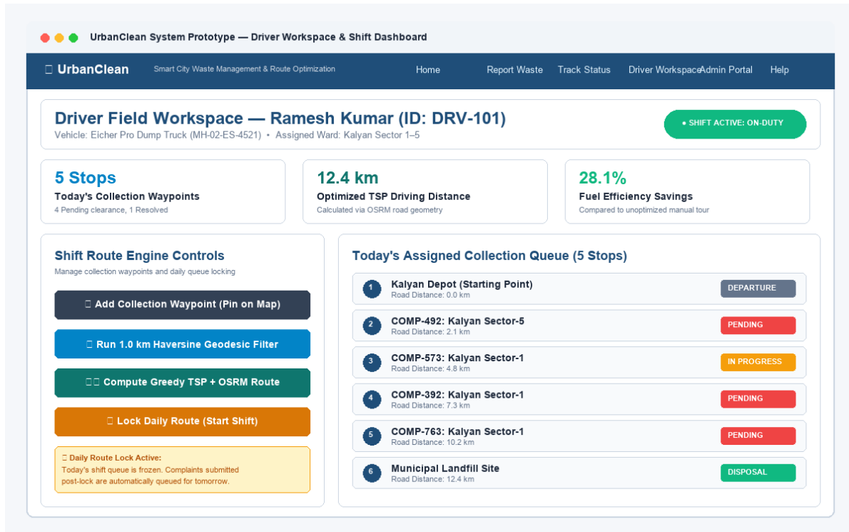
Figure 5.7: Prototype — Waste Collection Driver Duty Dashboard
