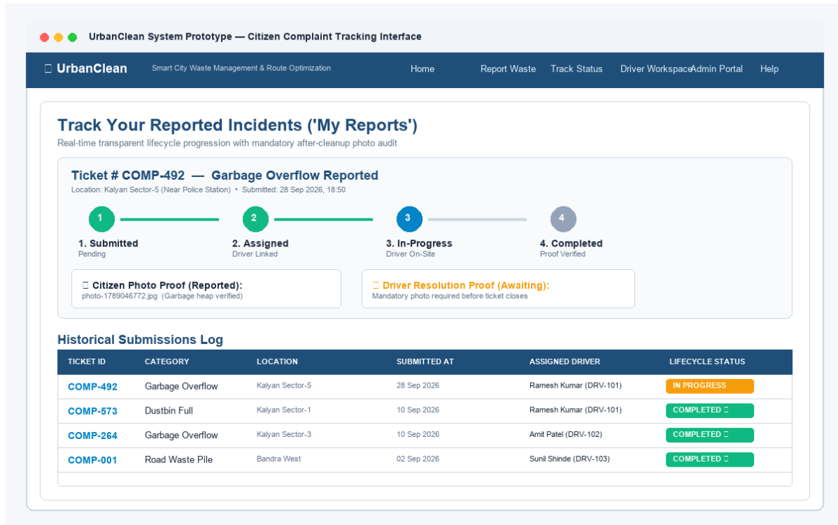
Figure 5.6: Prototype — Citizen Real-Time Complaint Tracking & Lifecycle Dashboard
