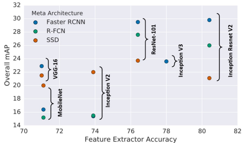
Fig. 13. Comparison of detection accuracy of three detectors: Faster RCNN [19], R-FCN [49], and SSD [23] on the MS-COCO dataset with different detection backbones. Image from CVPR 2017 [186].
