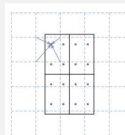
Figure 3. RoIAlign : The dashed grid represents a feature map, the solid lines an RoI (with 2 \times 2 bins in this example), and the dots the 4 sampling points in each bin. RoIAlign computes the value of each sampling point by bilinear interpolation from the nearby grid points on the feature map. No quantization is performed on any coordinates involved in the RoI, its bins, or the sampling points.
