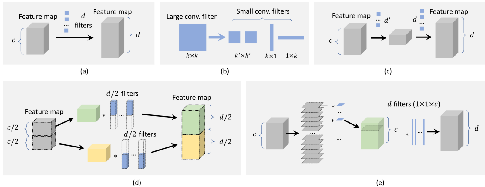
Fig. 10. Overview of speedup methods of a CNN's convolutional layer and the comparison of their computational complexity. (a) Standard convolution: \mathcal{O}(dk^2c) . (b) Factoring convolutional filters ( k \times k \rightarrow (k' \times k')^2 or 1 \times k, k \times 1 ): \mathcal{O}(dk'^2c) or \mathcal{O}(dkc) . (c) Factoring convolutional channels: \mathcal{O}(d'k^2c) + \mathcal{O}(dk^2d') . (d) Group convolution (#groups = m ): \mathcal{O}(dk^2c/m) . (e) Depthwise separable convolution: \mathcal{O}(ck^2) + \mathcal{O}(dc) .
