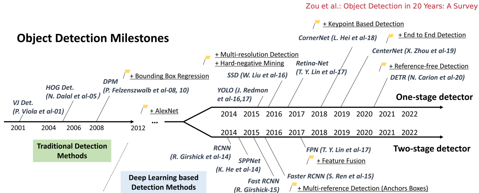
Fig. 2. Road map of object detection. Milestone detectors in this figure: VJ Det. [10], [11], HOG Det. [12], DPM [13], [14], [15], RCNN [16], SPPNet [17], Fast RCNN [18], Faster RCNN [19], YOLO [20], [21], [22], SSD [23], FPN [24], Retina-Net [25], CornerNet [26], CenterNet [27], and DETR [28].
