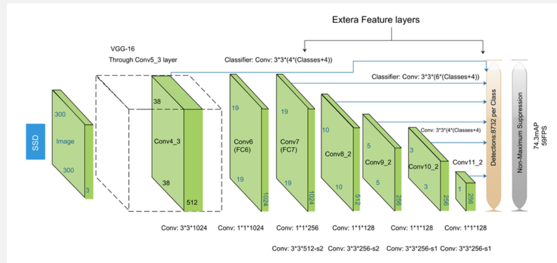
Figure 4. Single Shot Multi-Box Detector (SSD) architecture
