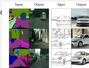
Fig. 12. Examples of images generated by applying pix2pix to synthesize street scenes from semantic maps (left) in the cityscapes dataset [84], and to create car images from edges (right). The input column presents the images x_A inserted into the generator, while the corresponding generated images G(x_A) are presented on the output column.
