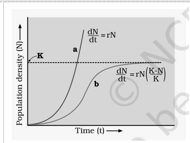
Fig. 11.3 - Population growth curve: a exponential, b logistic, K carrying capacity.
