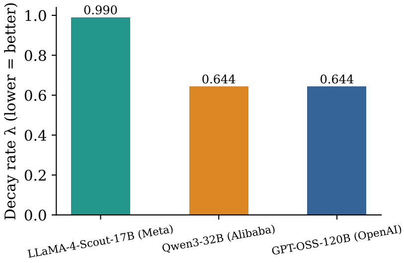
Fig 2 — Decay rate \lambda by model (RQ2)
