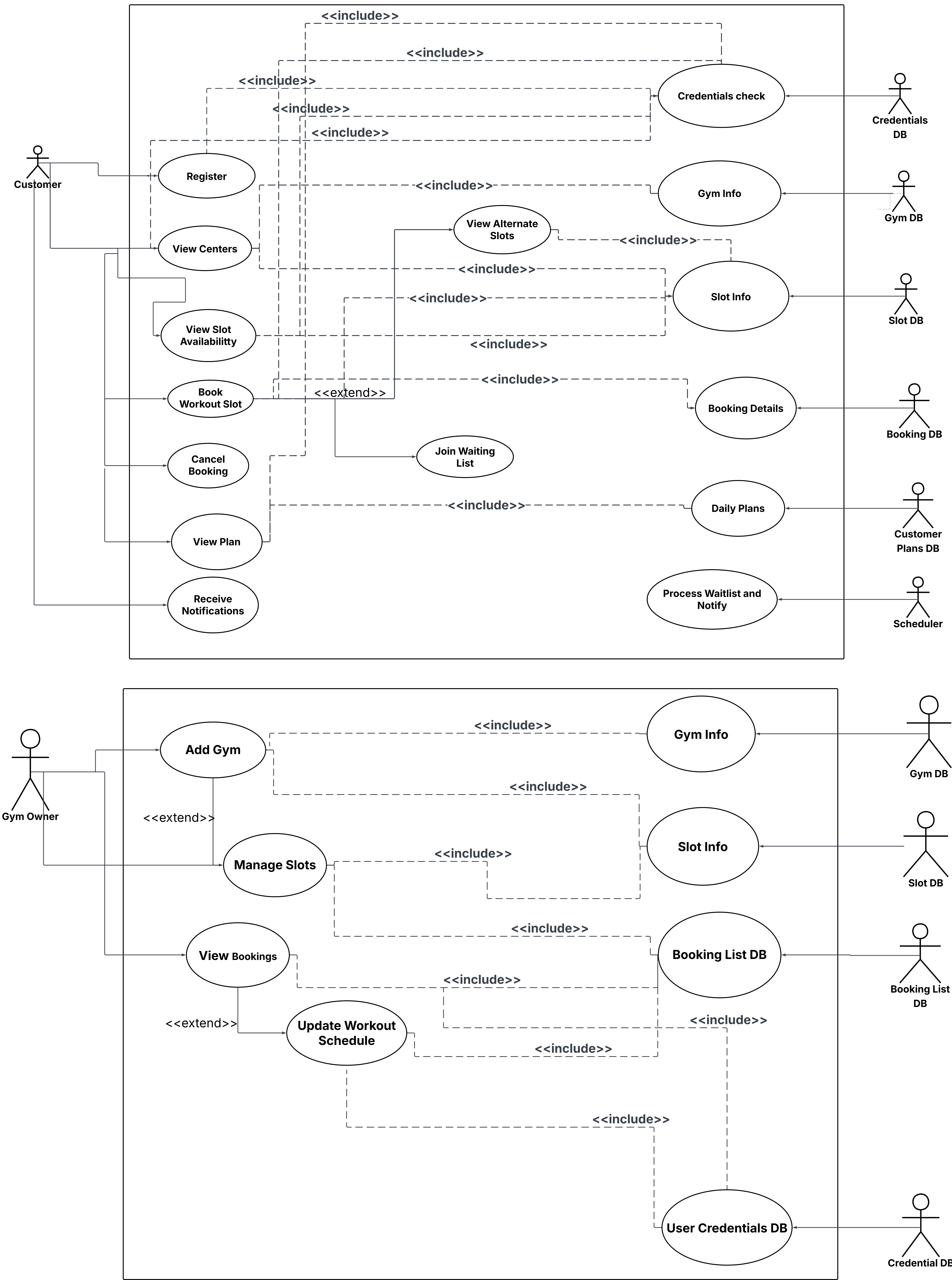
FlipFit Use Case Diagram
