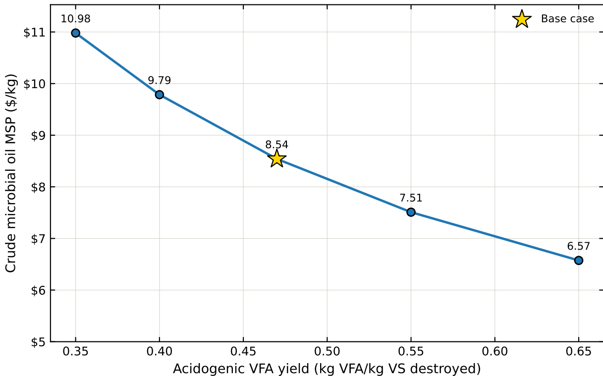
Effect of acidogenic VFA yield on crude microbial oil MSP
