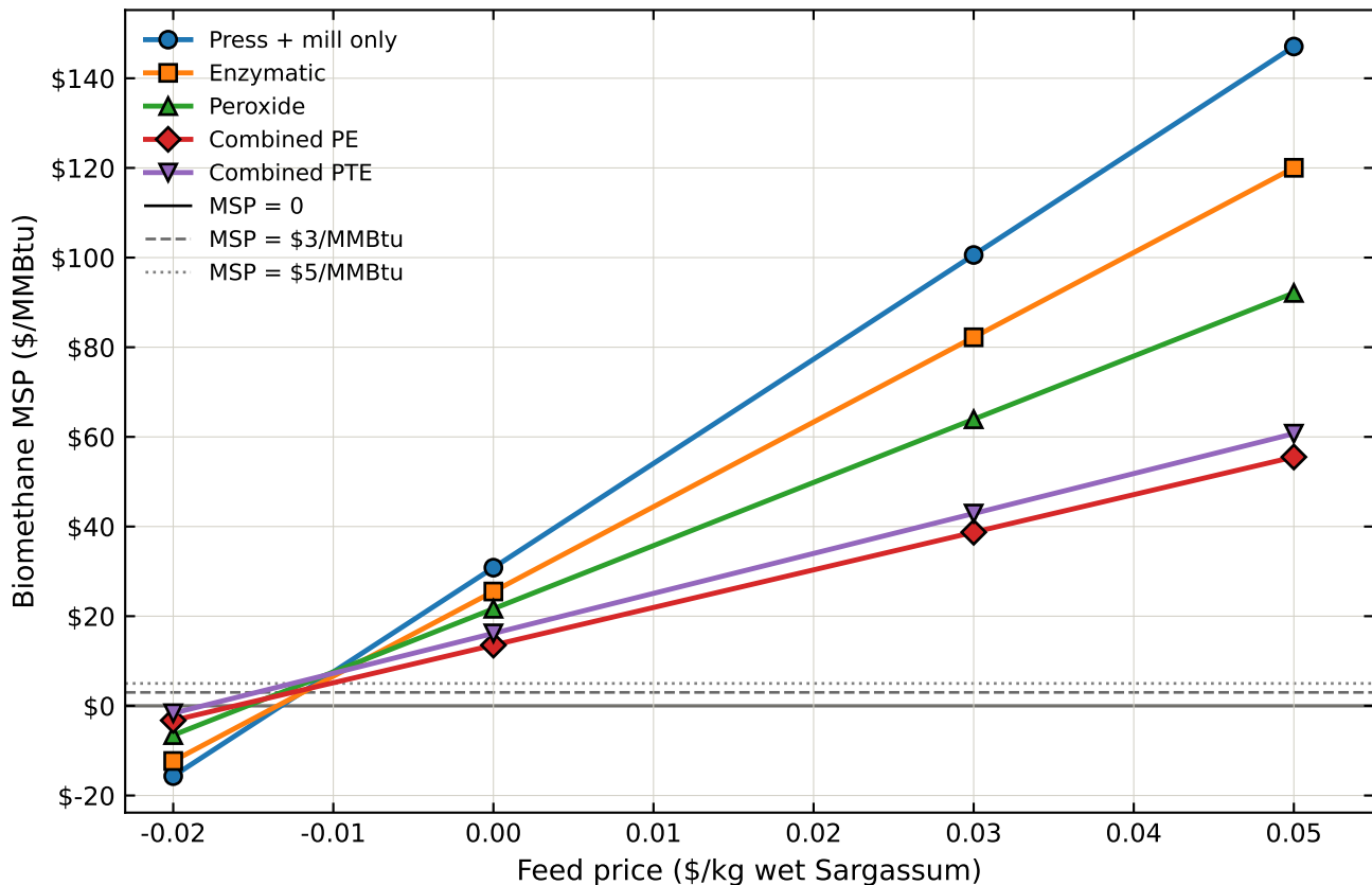
Effect of feed price on biomethane MSP across pretreatment cases
