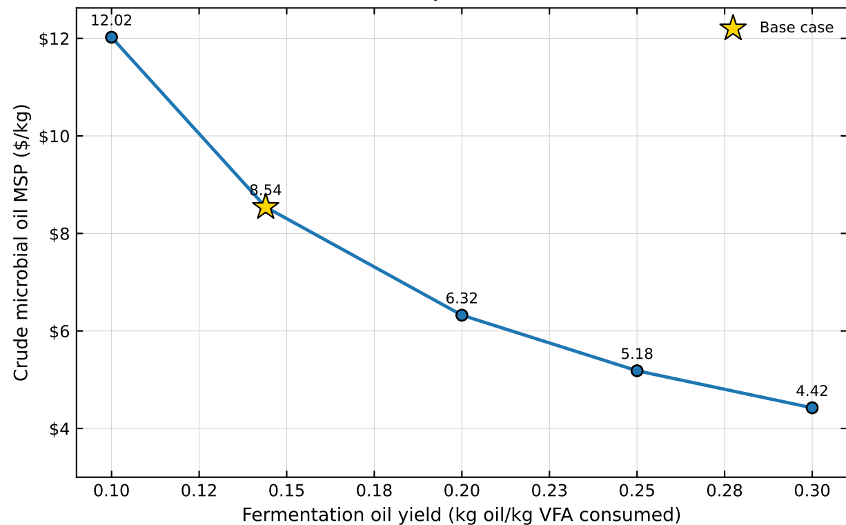
Effect of fermentation oil yield on crude microbial oil MSP
