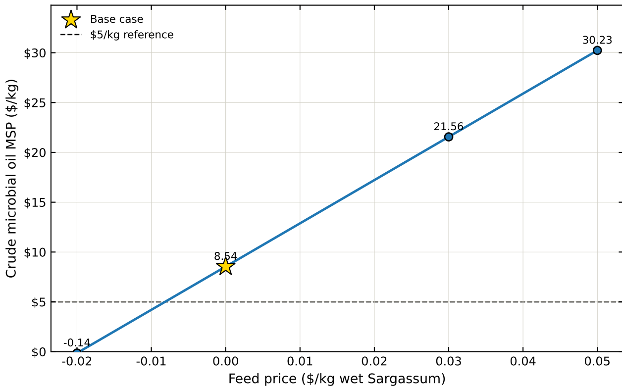
Effect of feed price on crude microbial oil MSP
