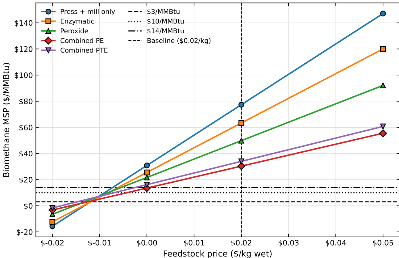
Effect of feedstock price on biomethane MSP
