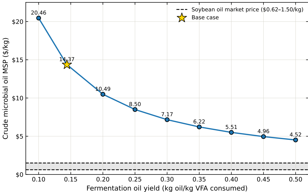
Effect of fermentation oil yield on crude microbial oil MSP
