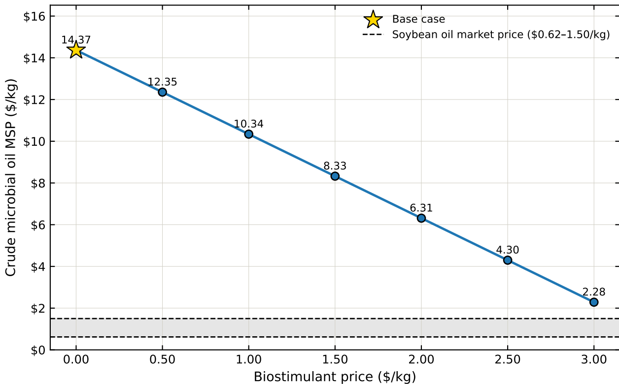
Effect of biostimulant price on crude microbial oil MSP
