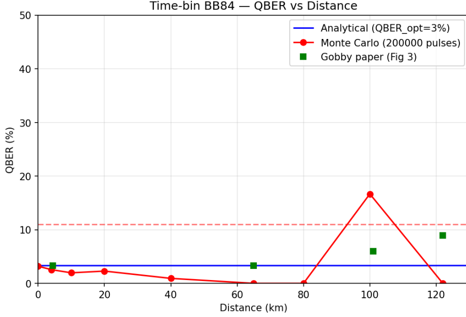
Figure 9: Time-bin BB84 validation against Gobby et al. (2004). Analytical curve (blue) with \text{QBER}_{\text{opt}} = 3.3\% and R_{\text{dc}} = 15 Hz. Monte Carlo points (red) from 200,000 pulses per distance (seed 42). Gobby paper data (green squares) from Fig. 3 [40]. The 0 km Monte Carlo QBER = 3.19% matches the paper’s \sim 3.3\% baseline. Statistical noise increases beyond 40 km due to limited sifted bits at \mu = 0.1 .
