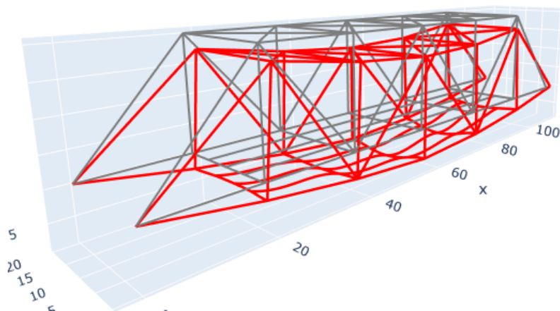
Figure. Extreme missing diagonals overload case, undeformed and deformed view.
