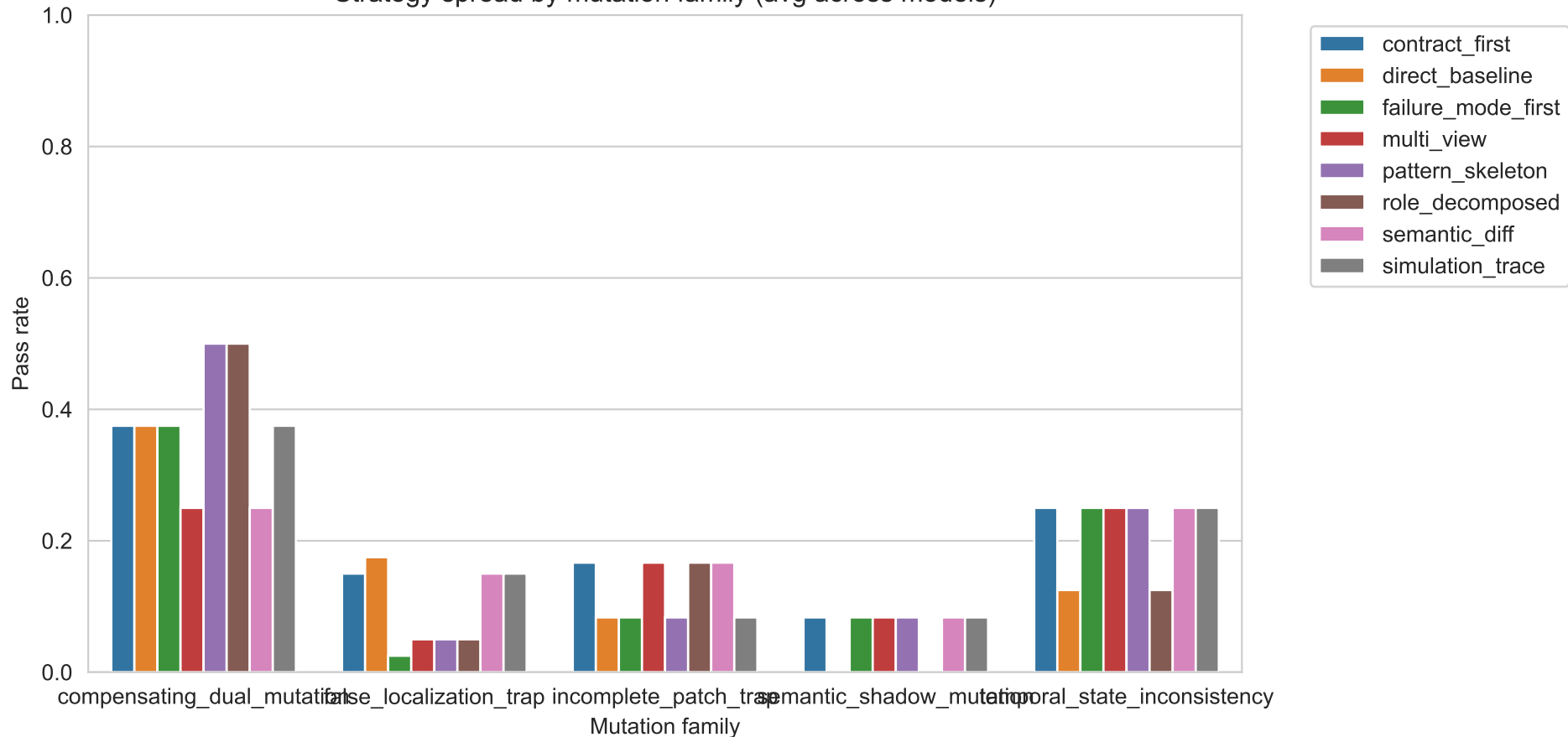
Strategy spread by mutation family (avg across models)
