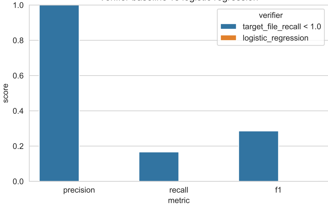
Verifier baseline vs logistic regression
