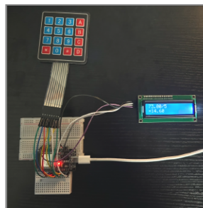
ESP32 Breadboard
