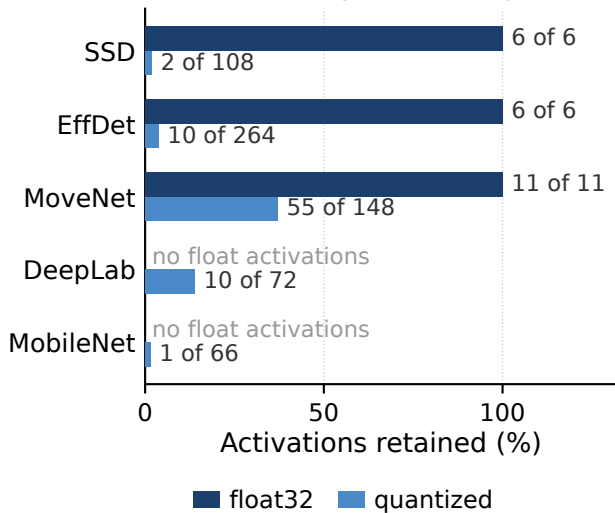
(a) Observability under delegation
