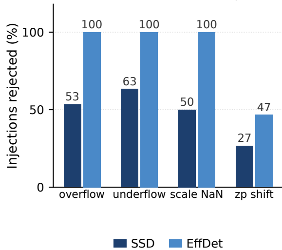
(b) Metadata validation, CPU path
