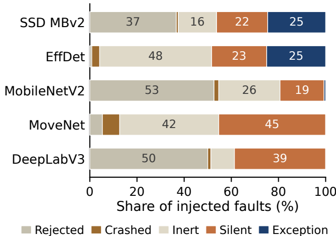
(b) Fault outcome composition
