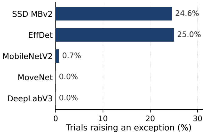
(a) Exception reachability
