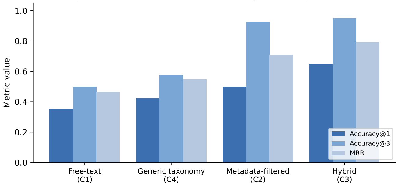
Synthetic retrieval simulation: ranking metrics by condition
